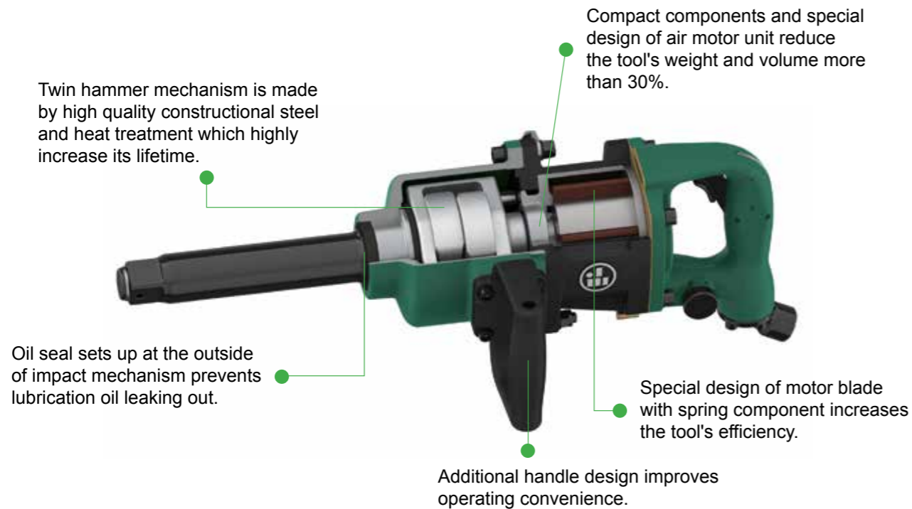
JAI-1408L 1" SQ. DR. Super Duty Air Impact Wrench W/8" Extended Anvil-----twin Hammer
