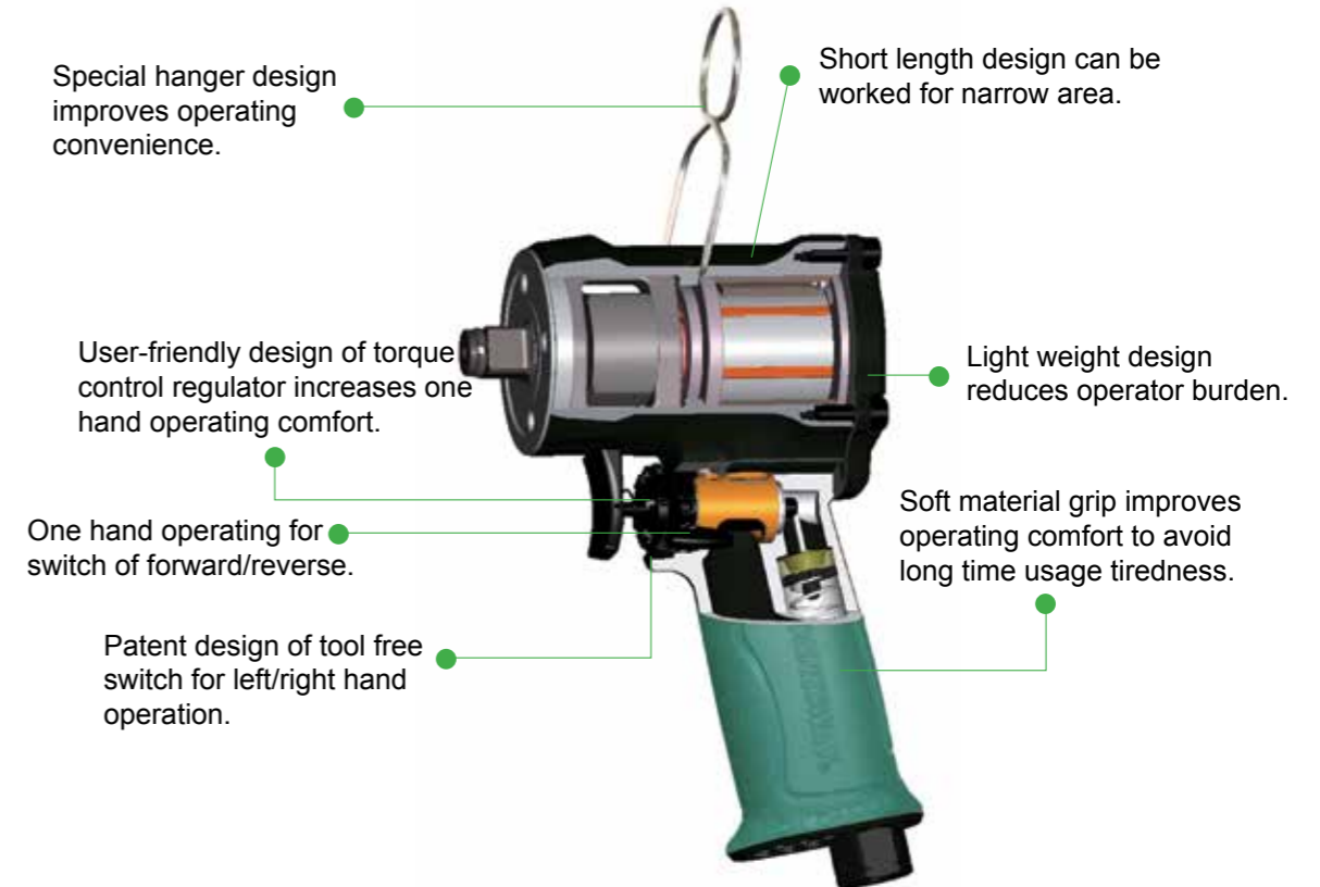
JAI-1014 1/2" Stubby Impact Wrench
